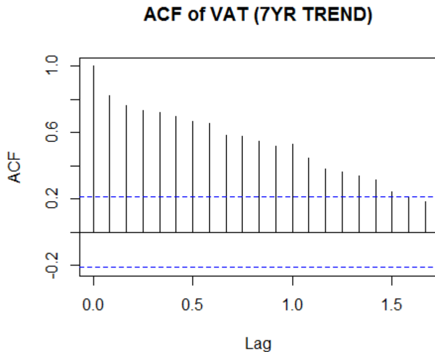
Figure 4.2: ACF of Monthly VAT Collections
