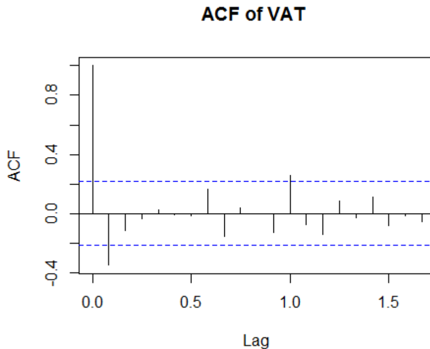
Figure 4.5: ACF of differenced VAT
